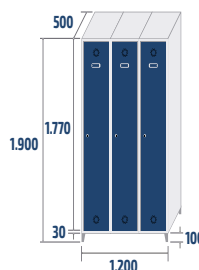
SV-40/3 COD: 44003 65kg · 1,14m 3
